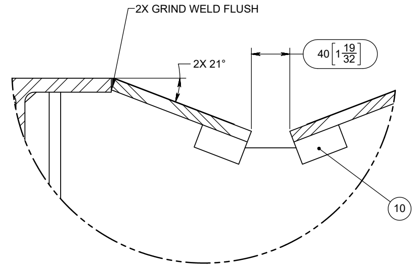
DETAIL F SCALE 1 : 2
