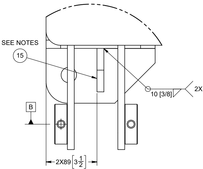
DETAIL G SCALE 1 : 2
